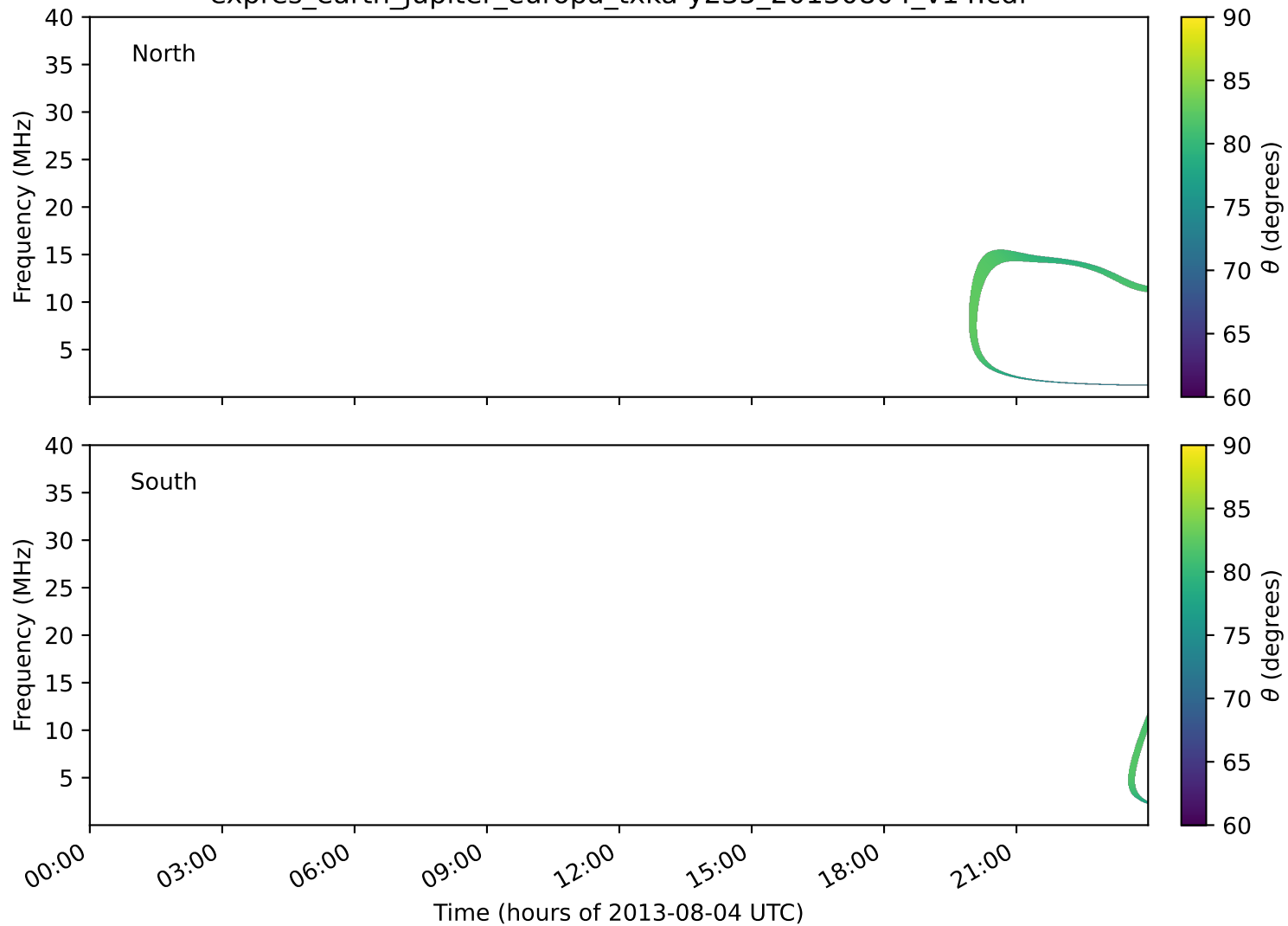
expres_earth_jupiter_europa_txka-y235_20130804_v14.cdf
