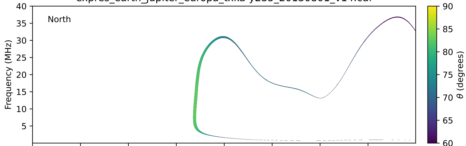
expres_earth_jupiter_europa_txka-y235_20130801_v14.cdf
