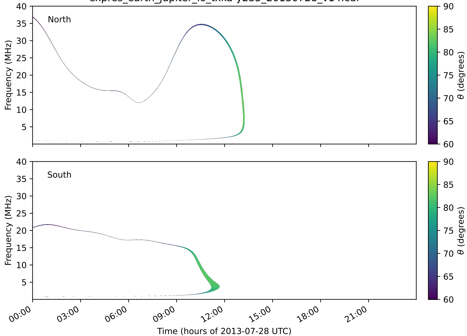
expres_earth_jupiter_io_txka-y235_20130728_v14.cdf
