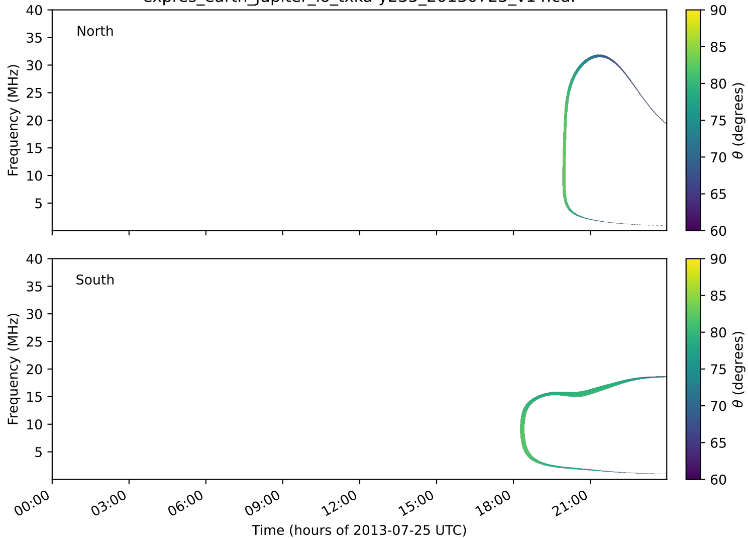
expres_earth_jupiter_io_txka-y235_20130725_v14.cdf
