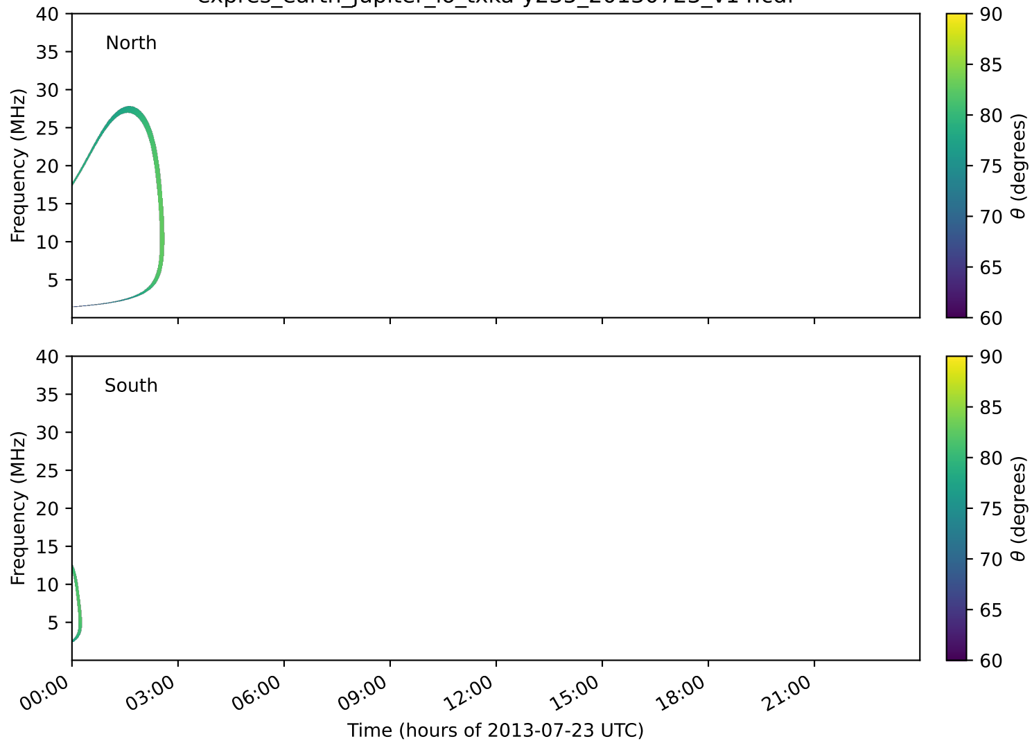
expres_earth_jupiter_io_txka-y235_20130723_v14.cdf
