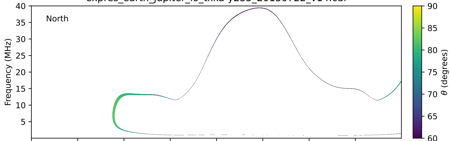
expres_earth_jupiter_io_txka-y235_20130722_v14.cdf
