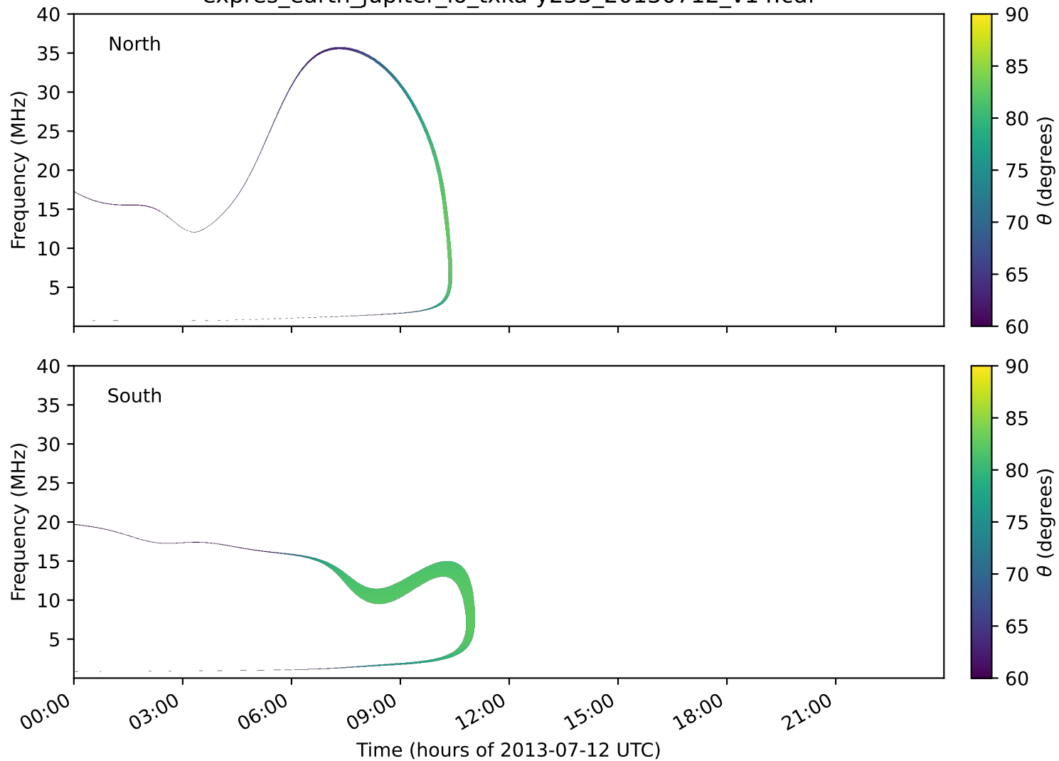
expres_earth_jupiter_io_txka-y235_20130712_v14.cdf
