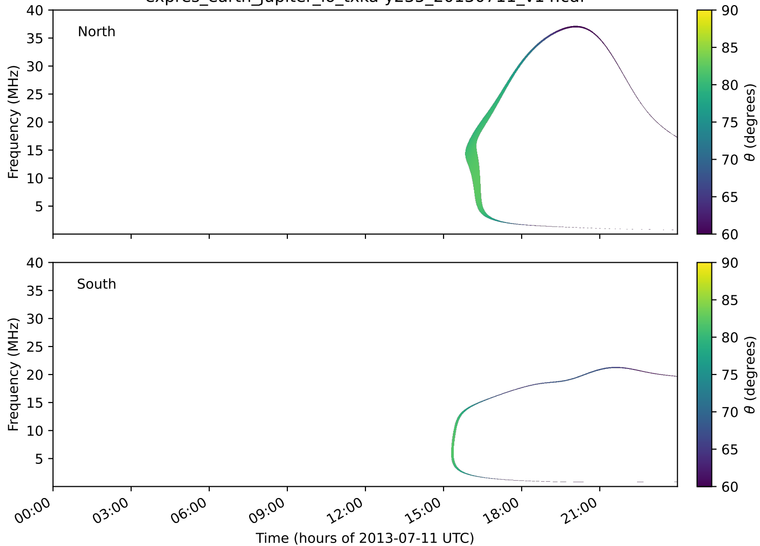
expres_earth_jupiter_io_txka-y235_20130711_v14.cdf
