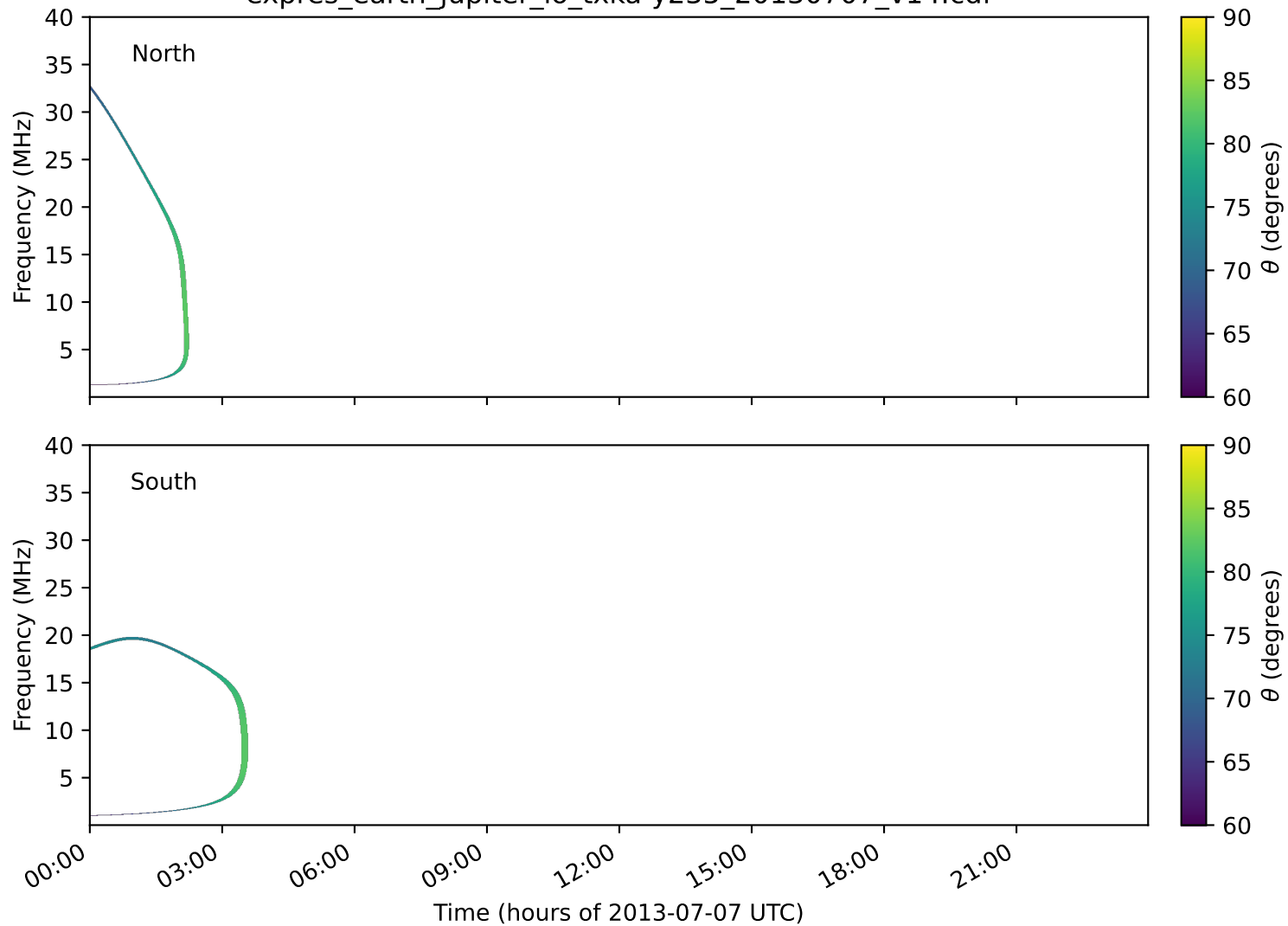
expres_earth_jupiter_io_txka-y235_20130707_v14.cdf
