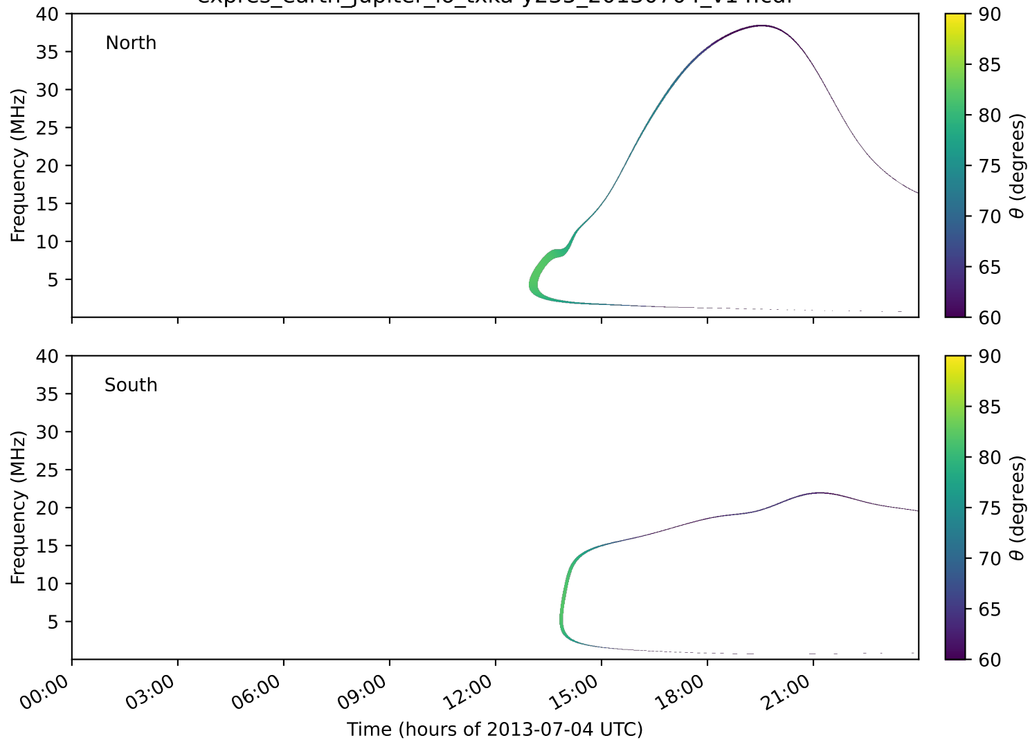
expres_earth_jupiter_io_txka-y235_20130704_v14.cdf
