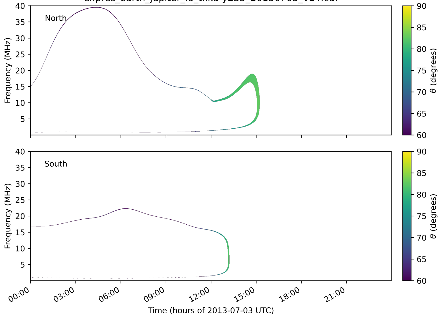
expres_earth_jupiter_io_txka-y235_20130703_v14.cdf
