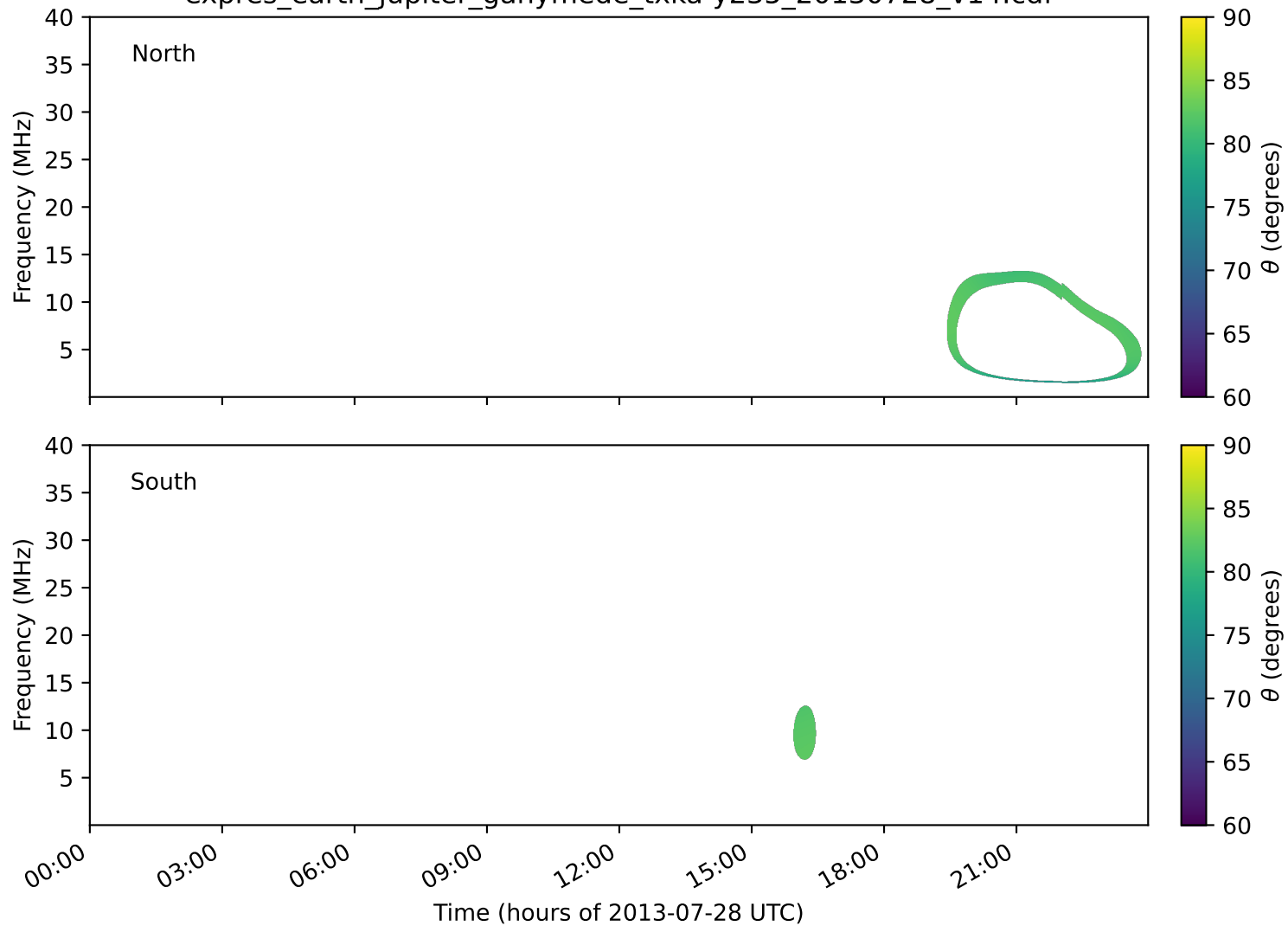
expres_earth_jupiter_ganymede_txka-y235_20130728_v14.cdf
