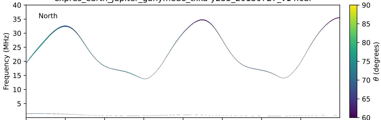
expres_earth_jupiter_ganymede_txka-y235_20130727_v14.cdf
