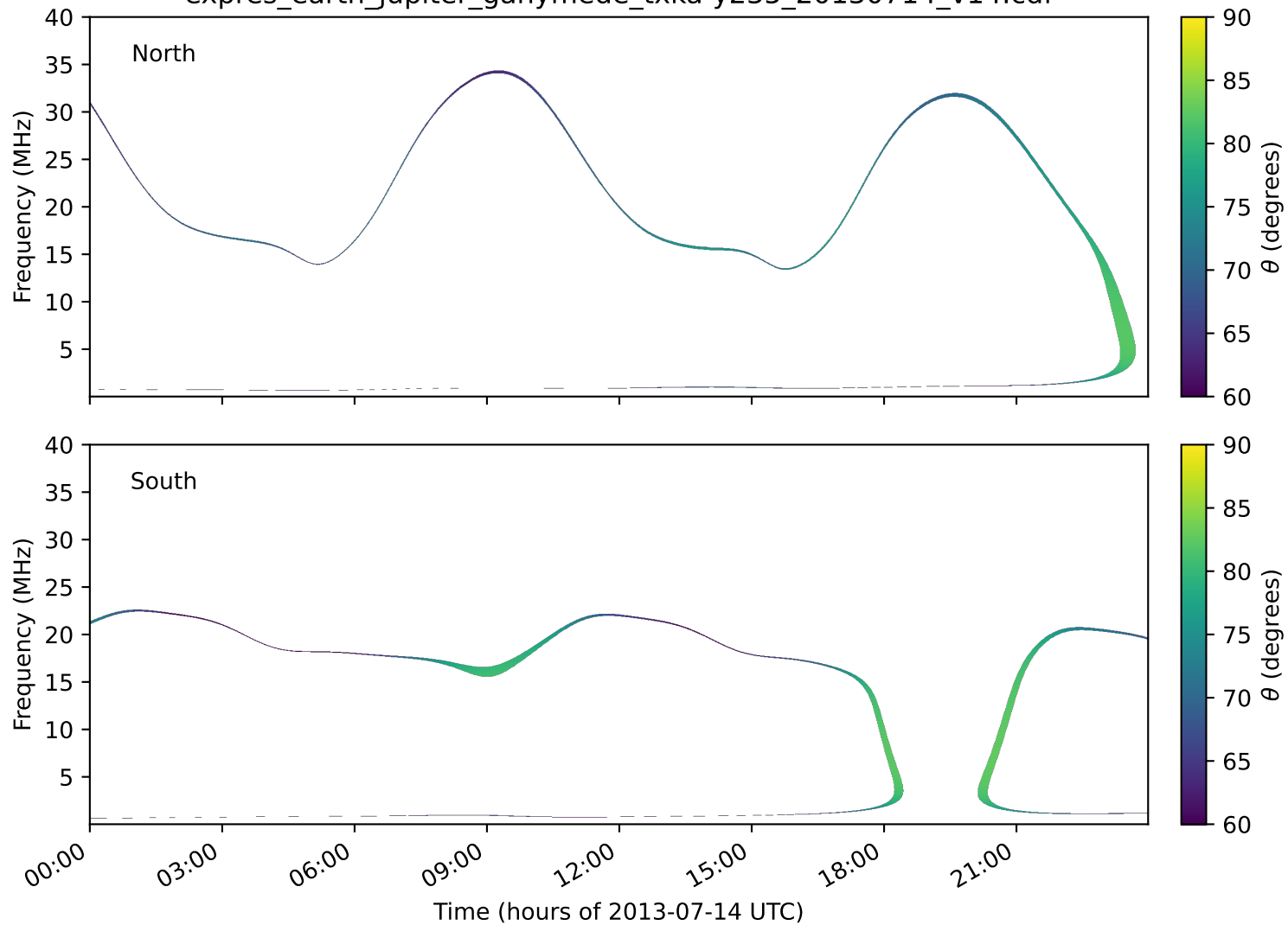
expres_earth_jupiter_ganymede_txka-y235_20130714_v14.cdf
