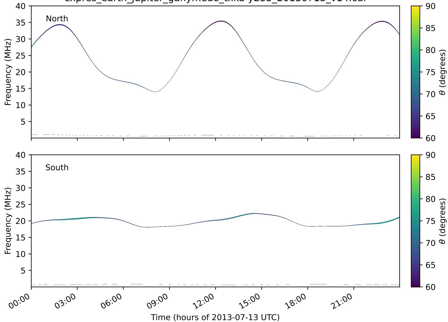
expres_earth_jupiter_ganymede_txka-y235_20130713_v14.cdf
