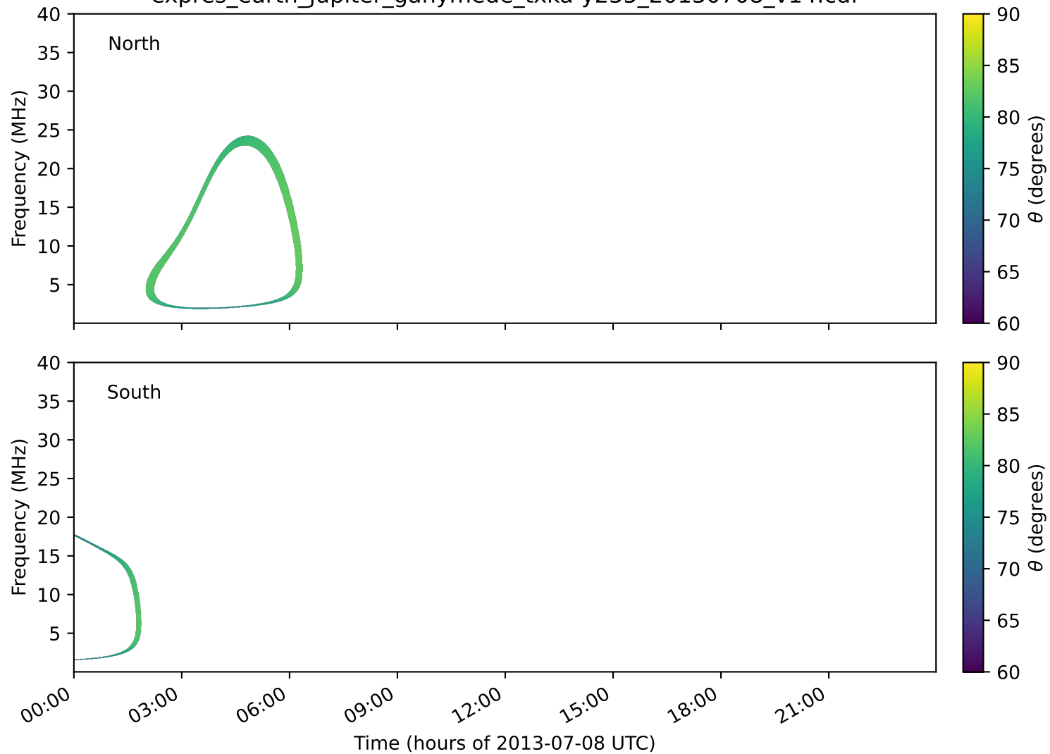
expres_earth_jupiter_ganymede_txka-y235_20130708_v14.cdf
