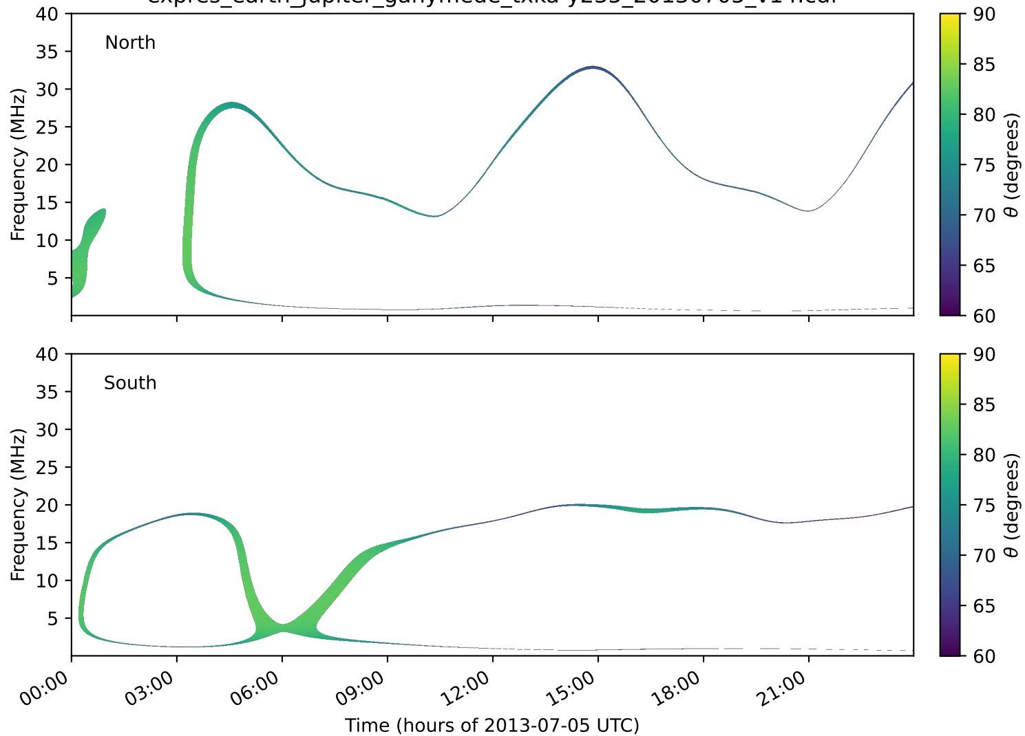
expres_earth_jupiter_ganymede_txka-y235_20130705_v14.cdf
