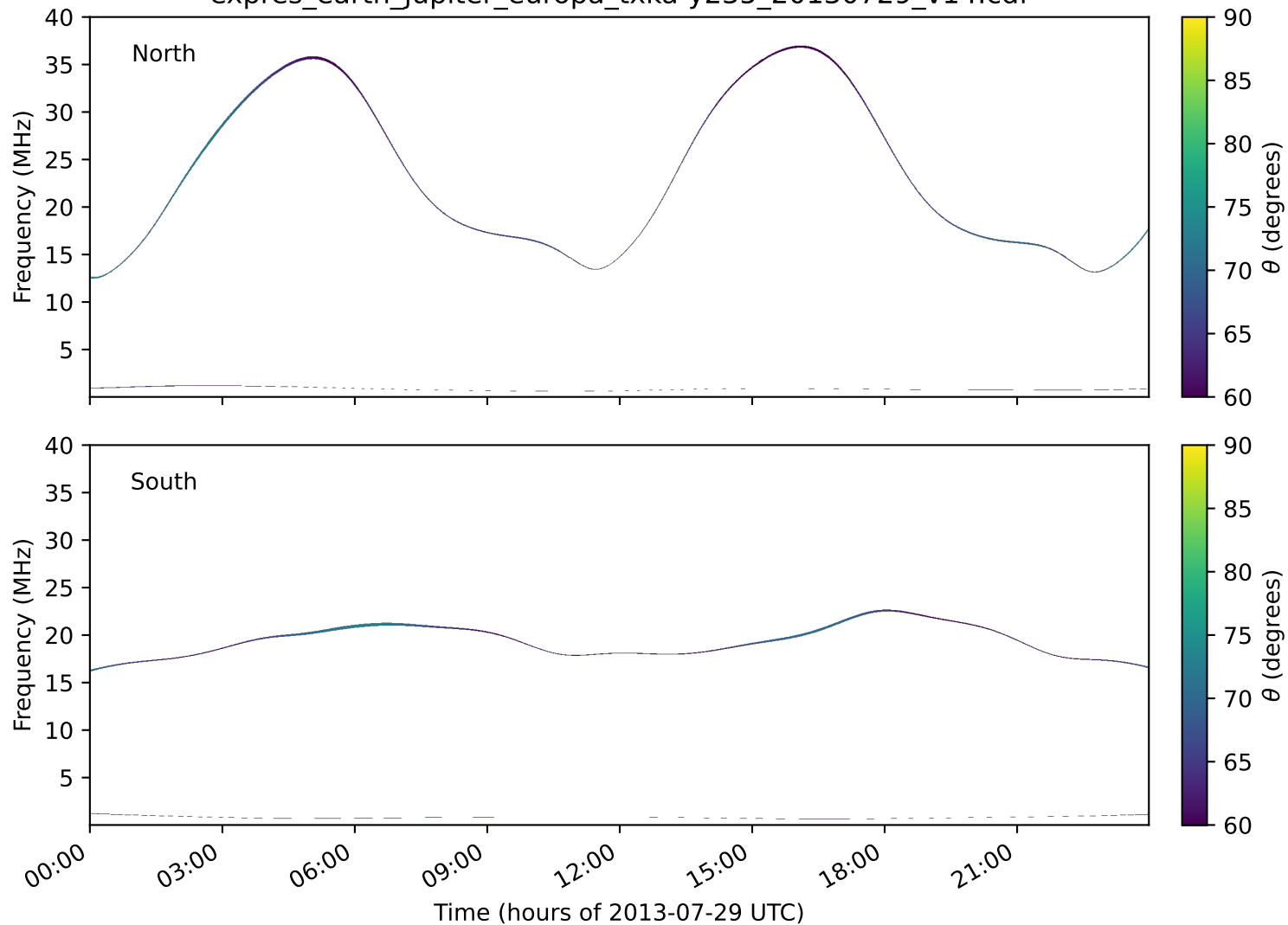
expres_earth_jupiter_europa_txka-y235_20130729_v14.cdf
