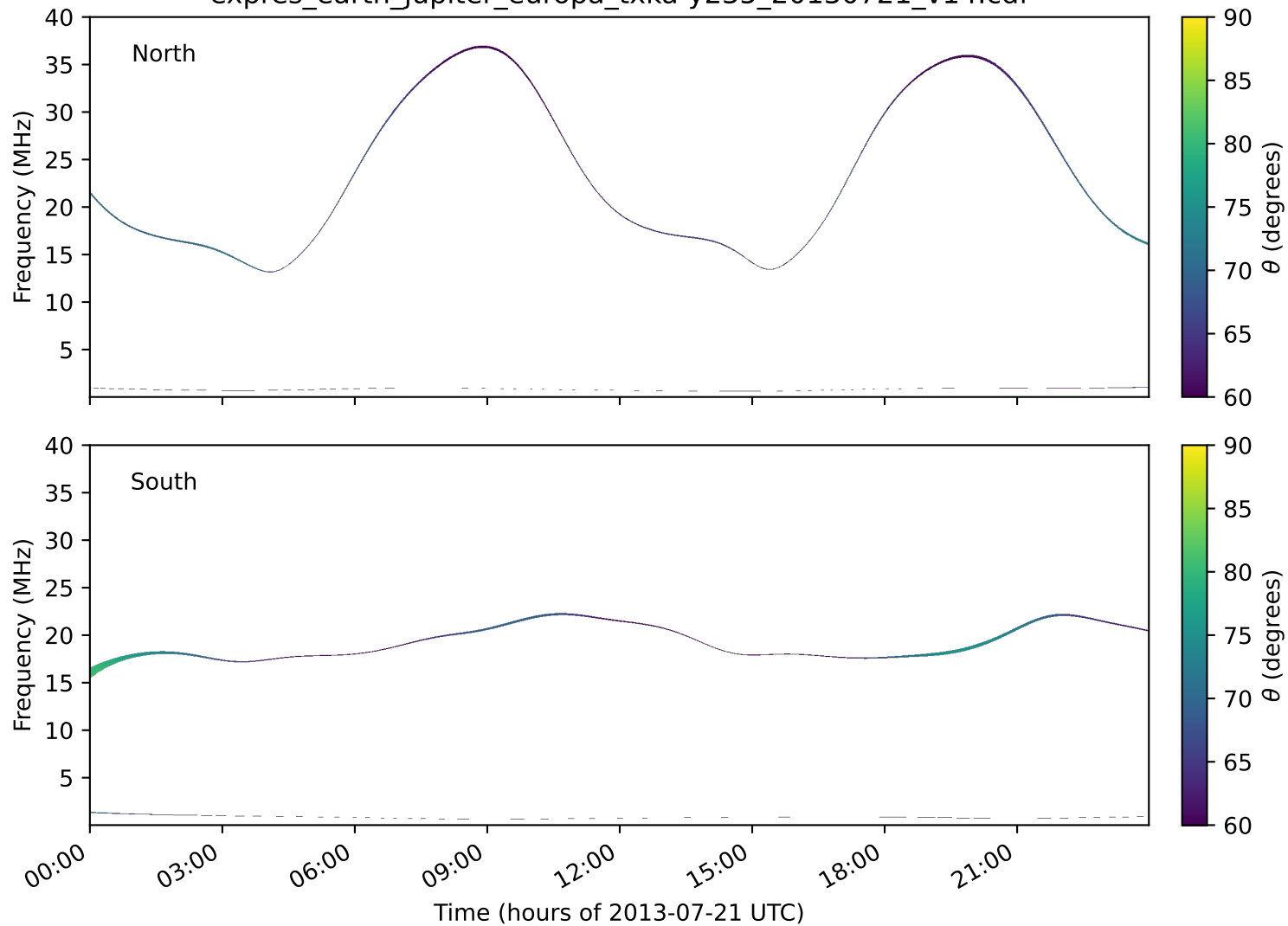
expres_earth_jupiter_europa_txka-y235_20130721_v14.cdf
