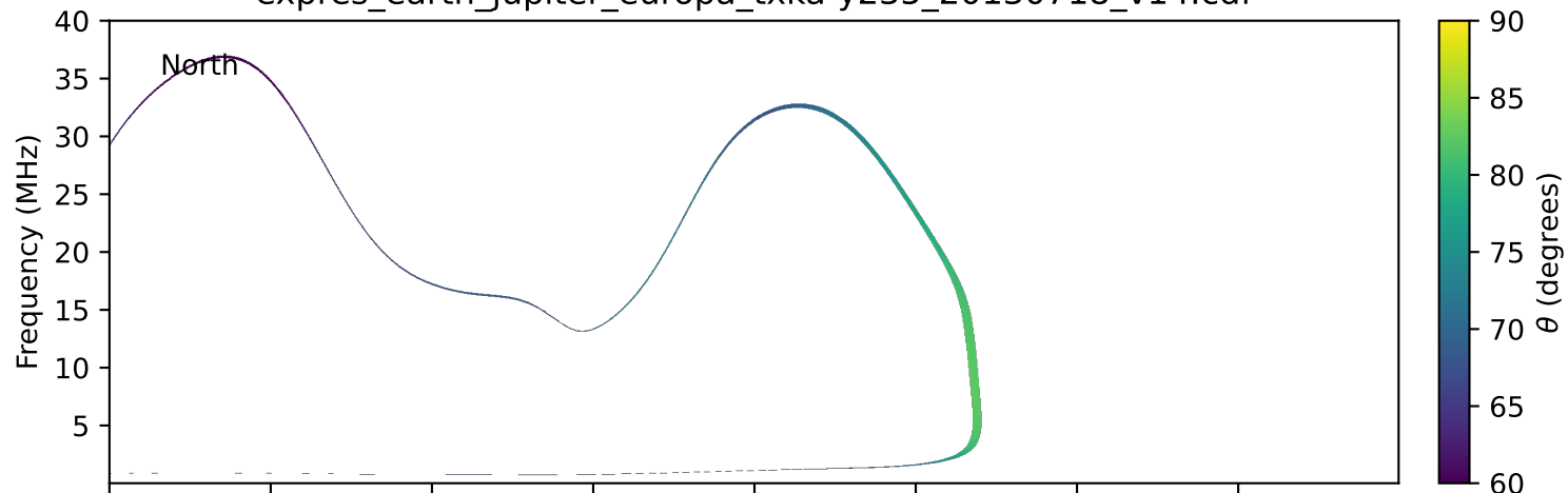
expres_earth_jupiter_europa_txka-y235_20130718_v14.cdf
