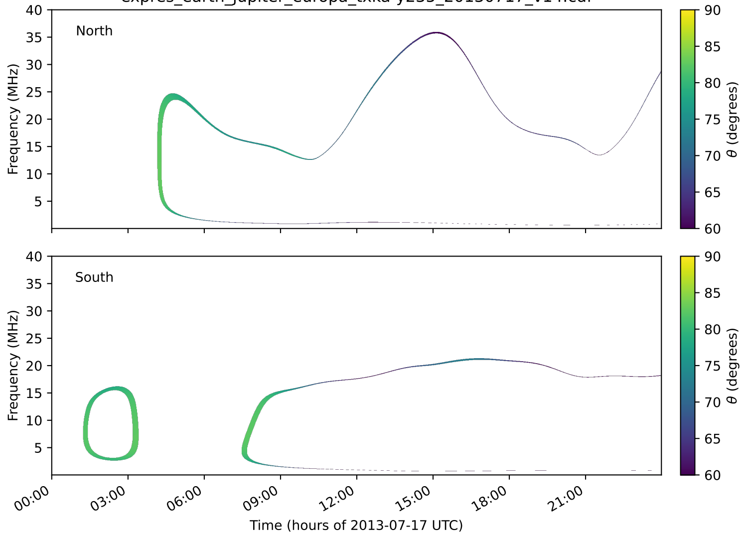
expres_earth_jupiter_europa_txka-y235_20130717_v14.cdf
