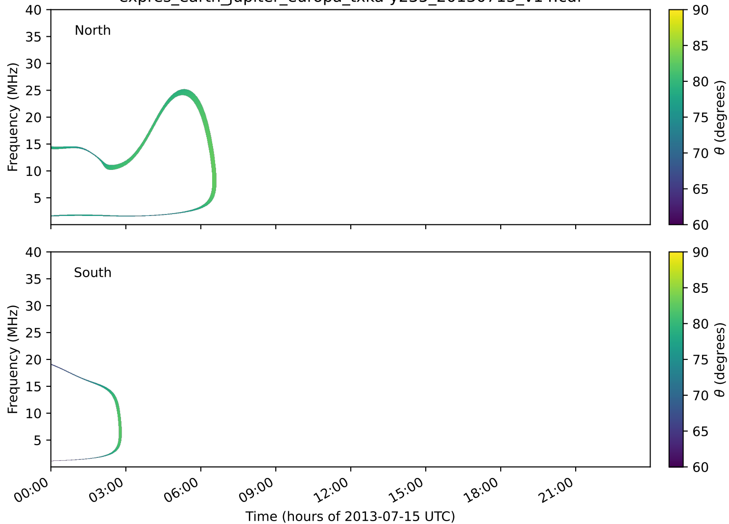
expres_earth_jupiter_europa_txka-y235_20130715_v14.cdf
