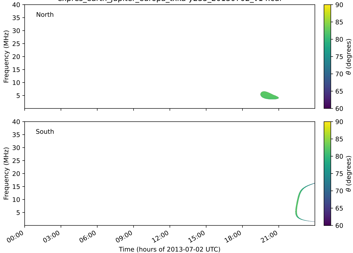
expres_earth_jupiter_europa_txka-y235_20130702_v14.cdf
