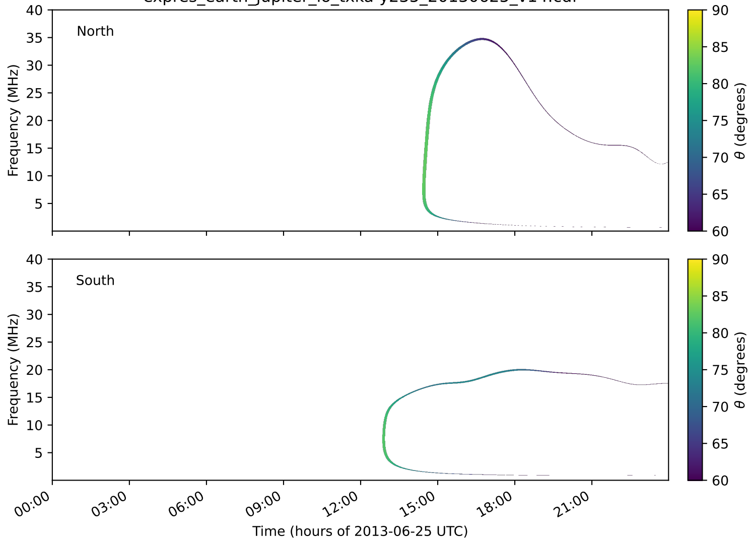
expres_earth_jupiter_io_txka-y235_20130625_v14.cdf
