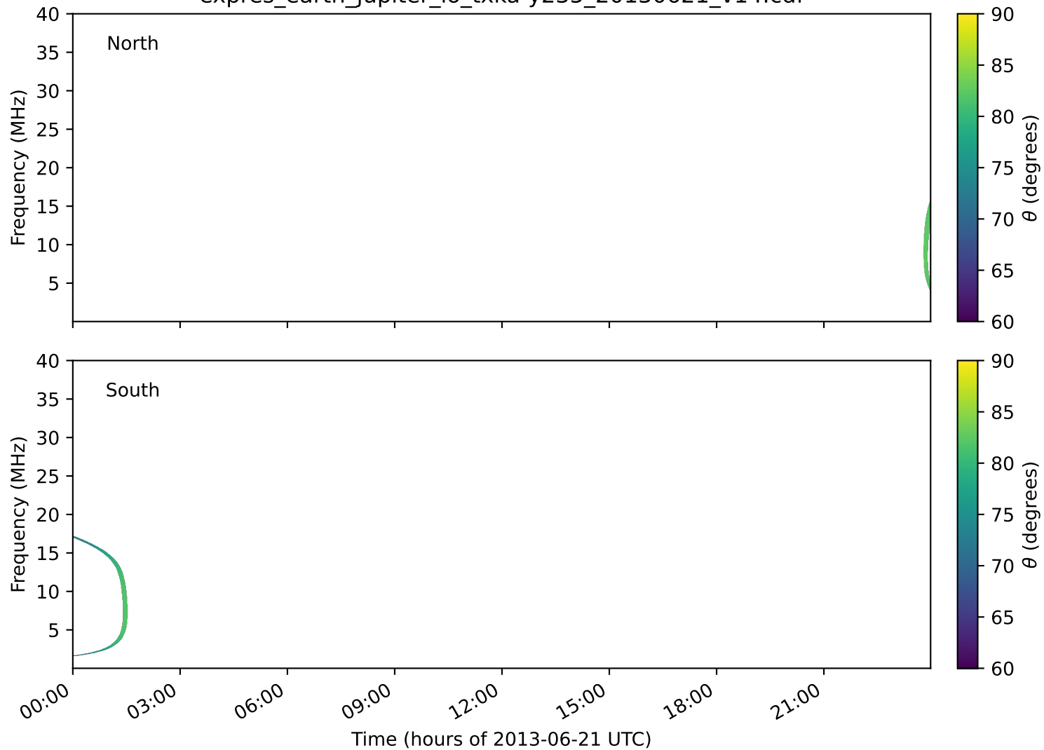
expres_earth_jupiter_io_txka-y235_20130621_v14.cdf
