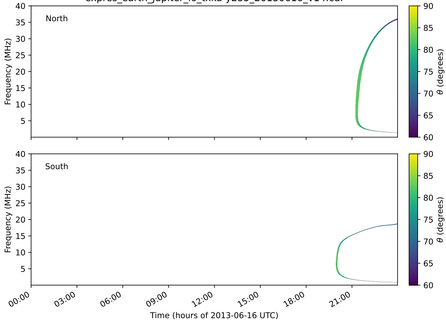
expres_earth_jupiter_io_txka-y235_20130616_v14.cdf
