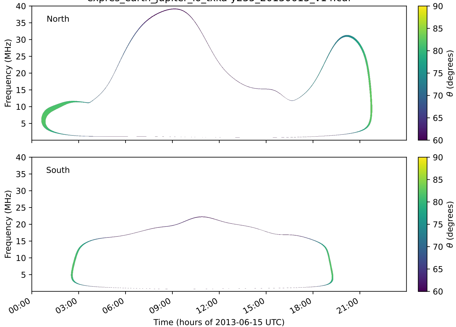
expres_earth_jupiter_io_txka-y235_20130615_v14.cdf
