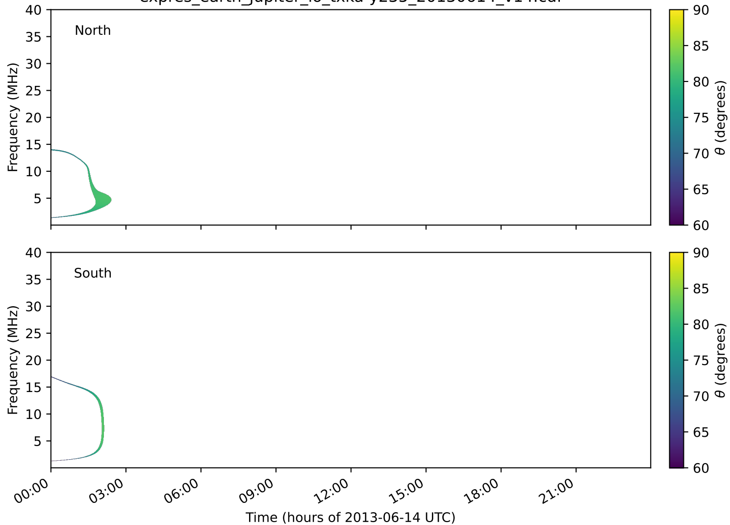
expres_earth_jupiter_io_txka-y235_20130614_v14.cdf
