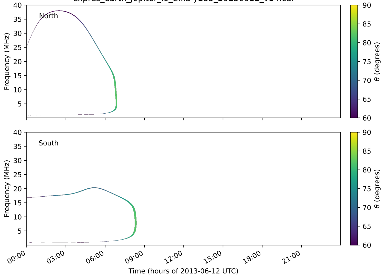
expres_earth_jupiter_io_txka-y235_20130612_v14.cdf
