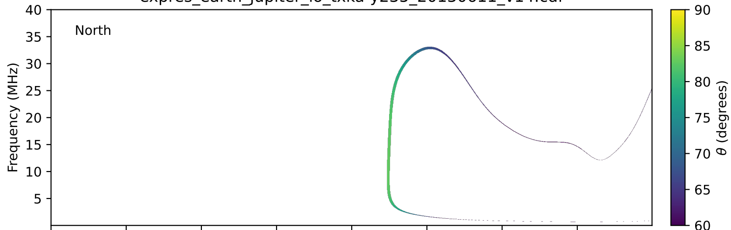
expres_earth_jupiter_io_txka-y235_20130611_v14.cdf
