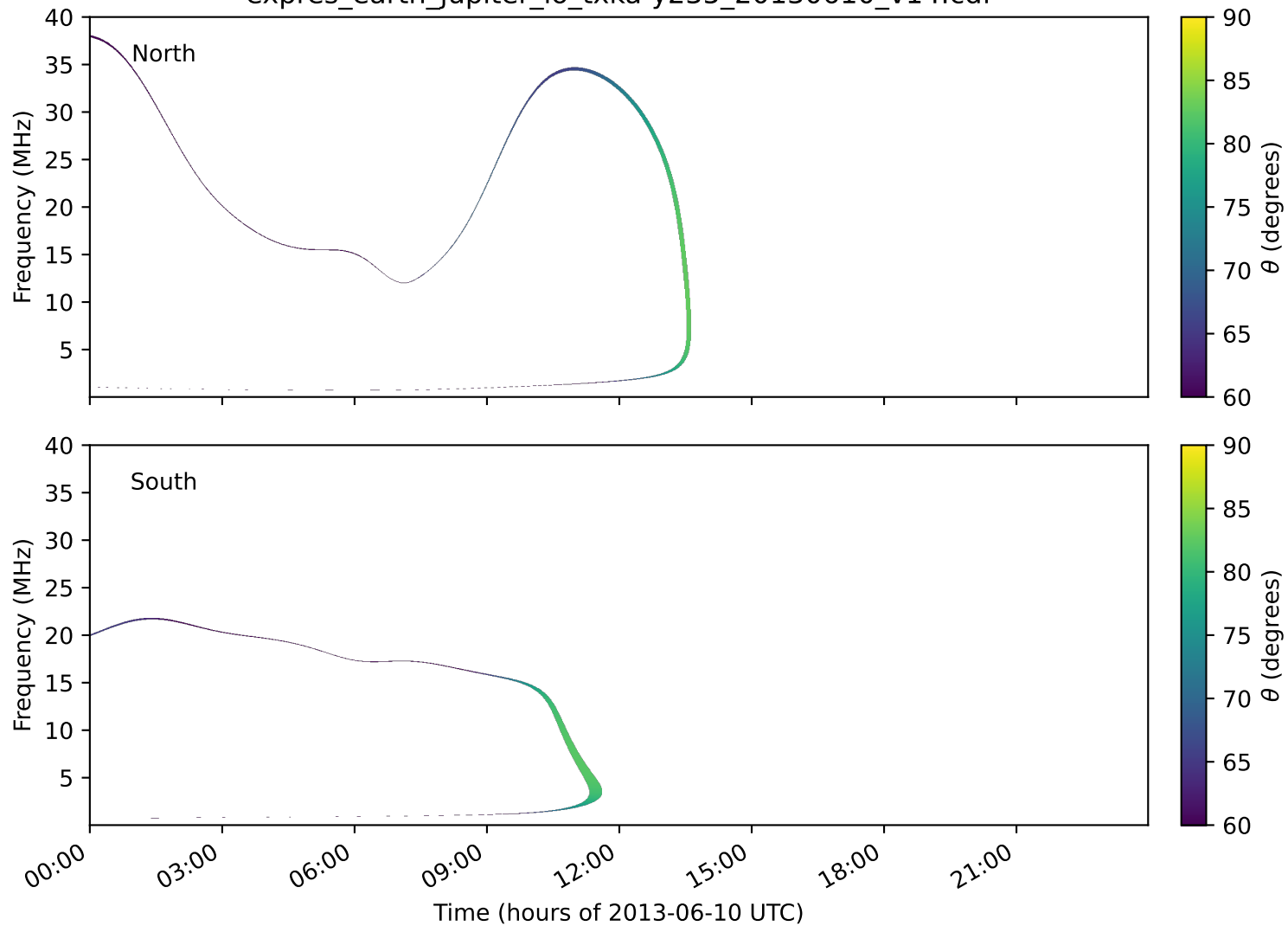
expres_earth_jupiter_io_txka-y235_20130610_v14.cdf
