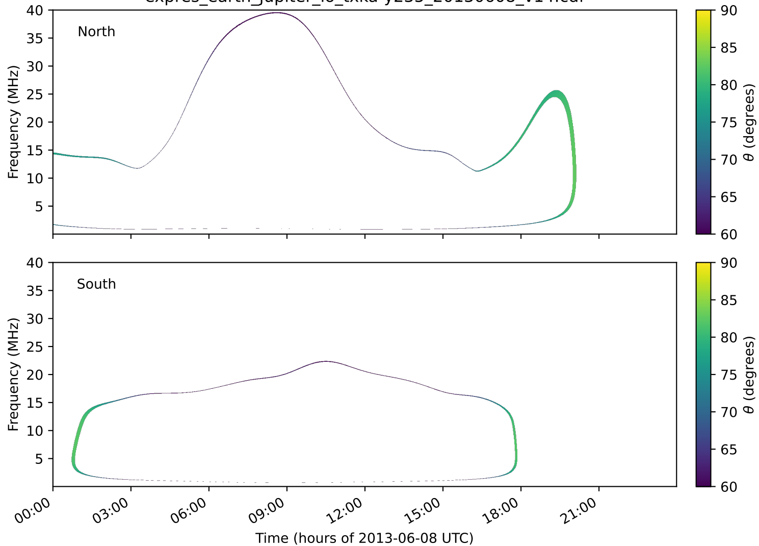
expres_earth_jupiter_io_txka-y235_20130608_v14.cdf
