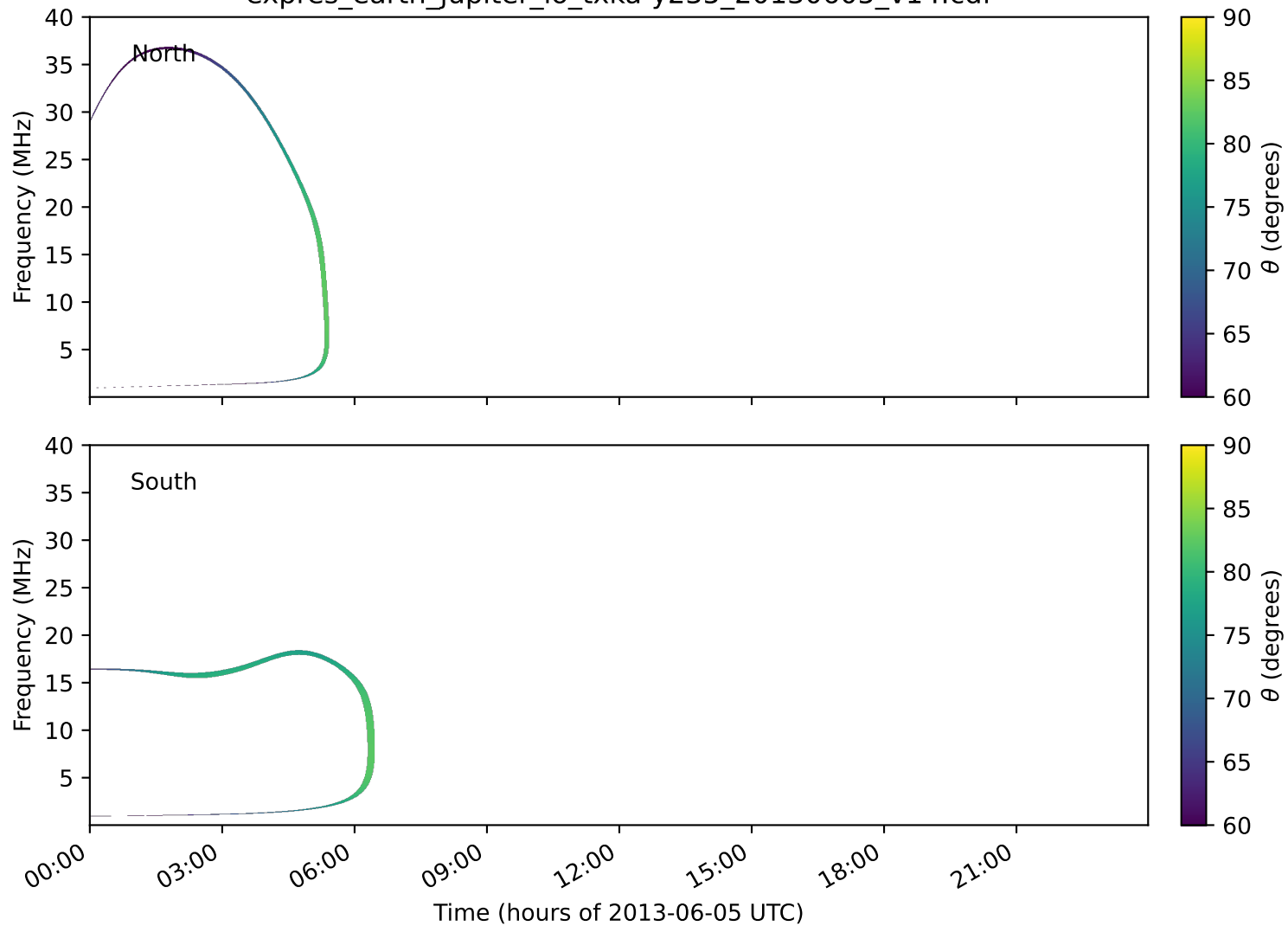
expres_earth_jupiter_io_txka-y235_20130605_v14.cdf
