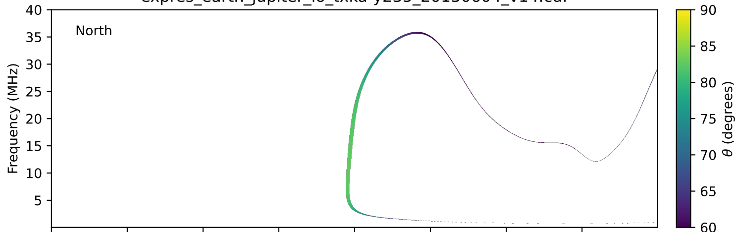
expres_earth_jupiter_io_txka-y235_20130604_v14.cdf
