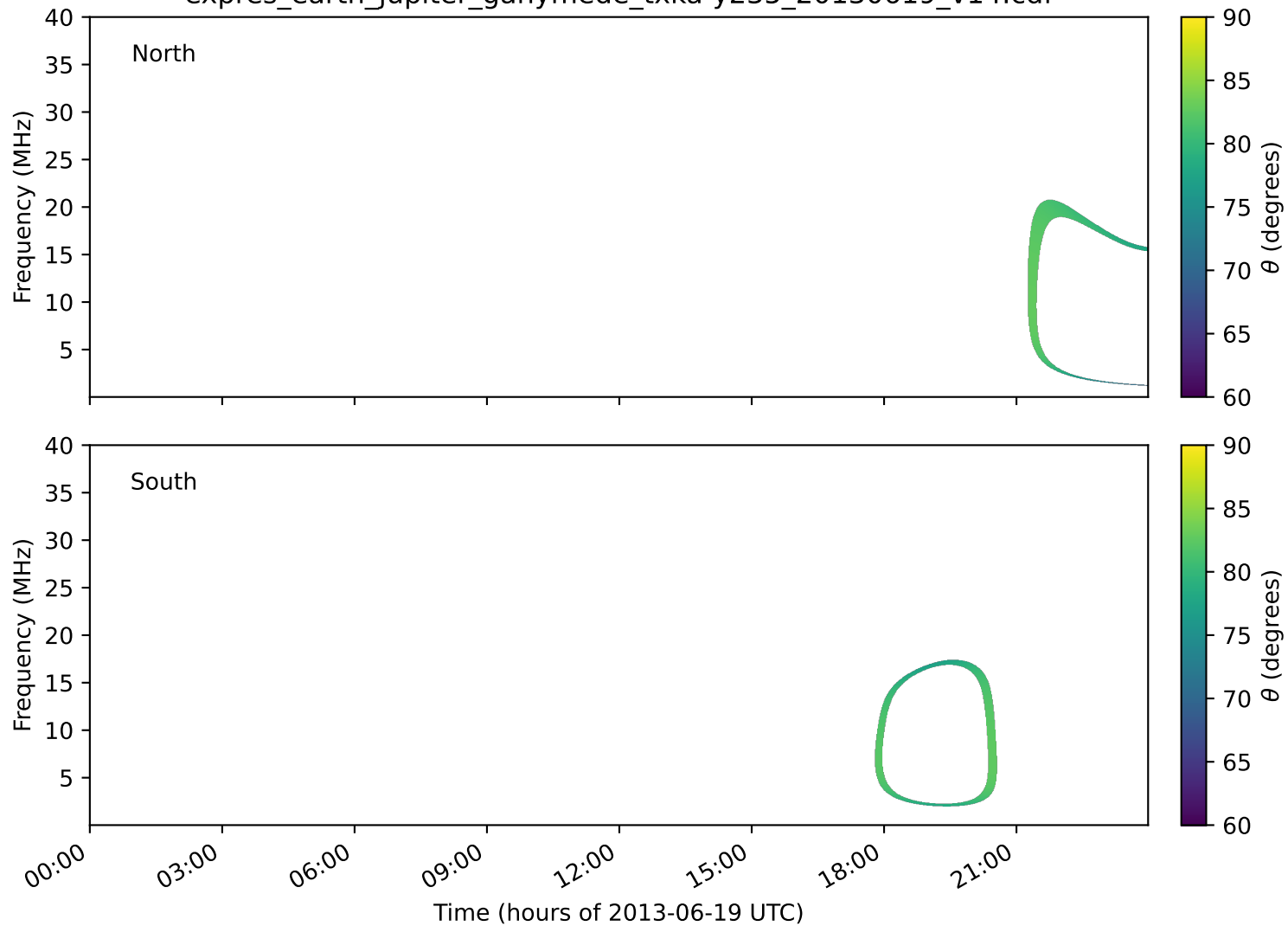
expres_earth_jupiter_ganymede_txka-y235_20130619_v14.cdf
