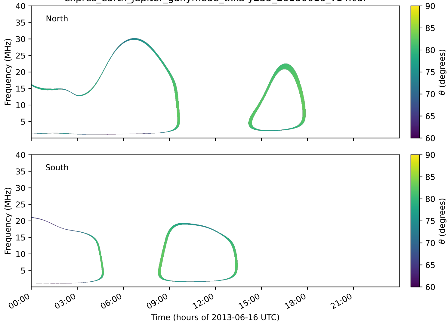
expres_earth_jupiter_ganymede_txka-y235_20130616_v14.cdf
