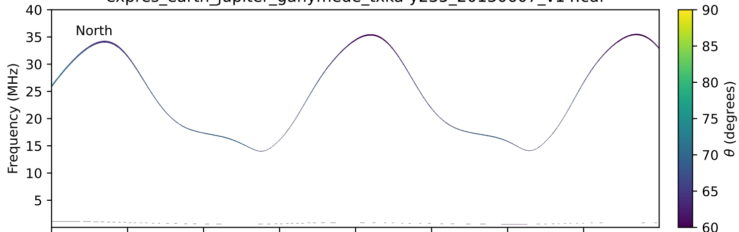
expres_earth_jupiter_ganymede_txka-y235_20130607_v14.cdf
