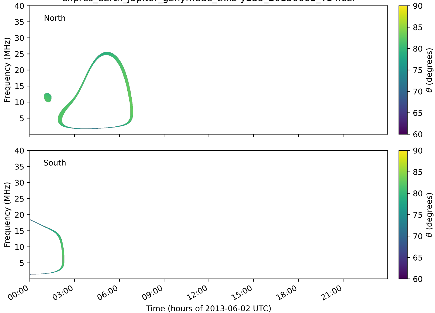
expres_earth_jupiter_ganymede_txka-y235_20130602_v14.cdf
