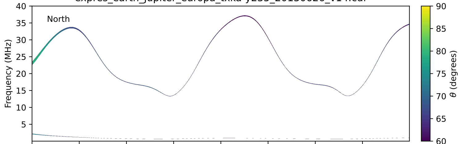
expres_earth_jupiter_europa_txka-y235_20130626_v14.cdf
