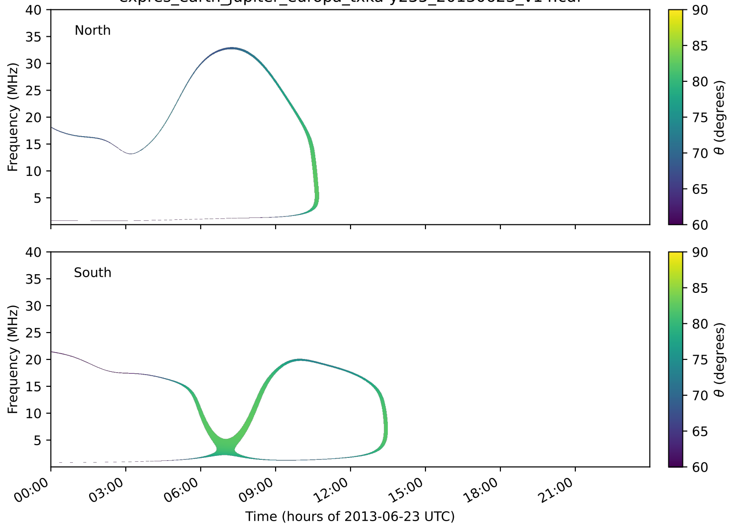
expres_earth_jupiter_europa_txka-y235_20130623_v14.cdf
