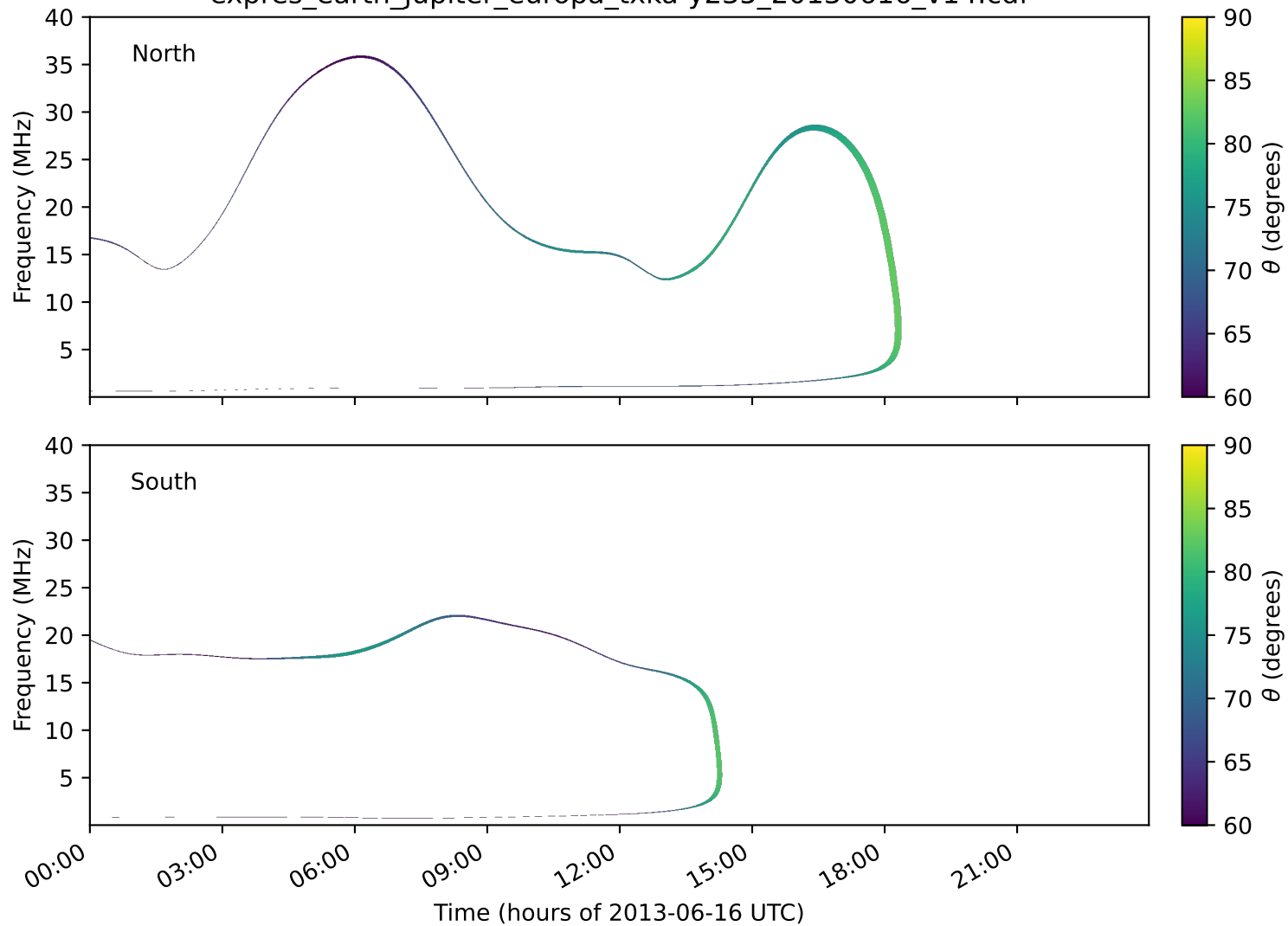
expres_earth_jupiter_europa_txka-y235_20130616_v14.cdf
