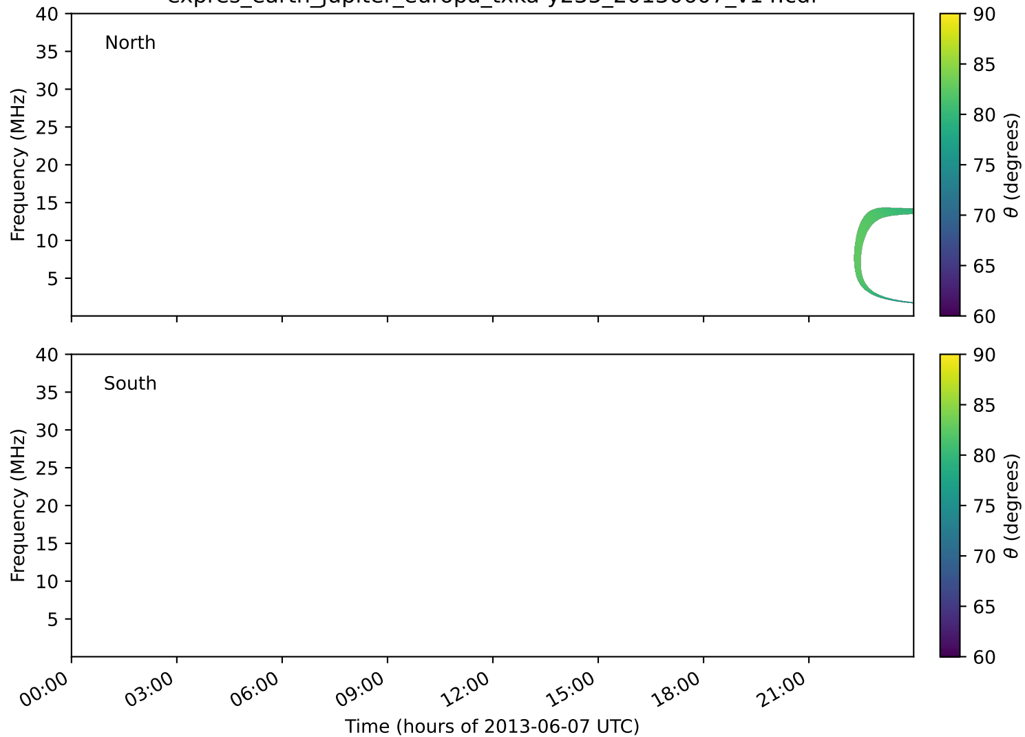
expres_earth_jupiter_europa_txka-y235_20130607_v14.cdf
