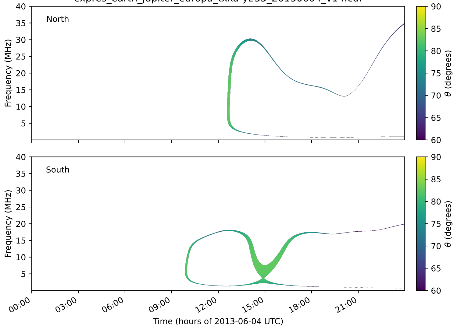
expres_earth_jupiter_europa_txka-y235_20130604_v14.cdf
