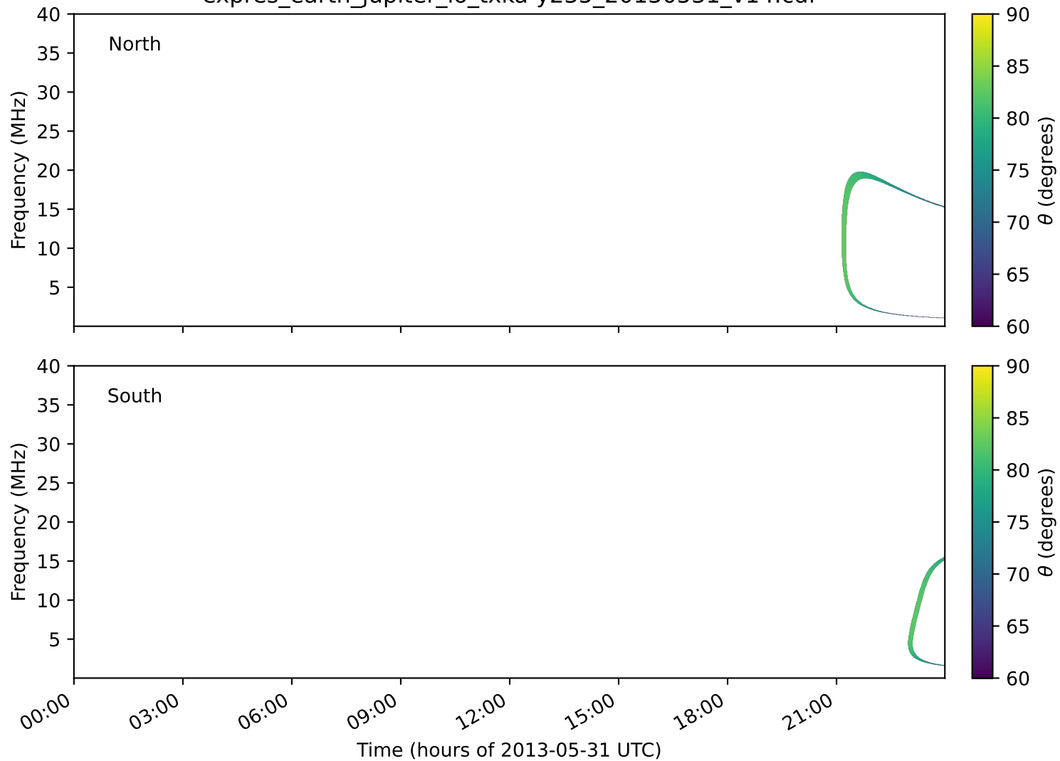
expres_earth_jupiter_io_txka-y235_20130531_v14.cdf
