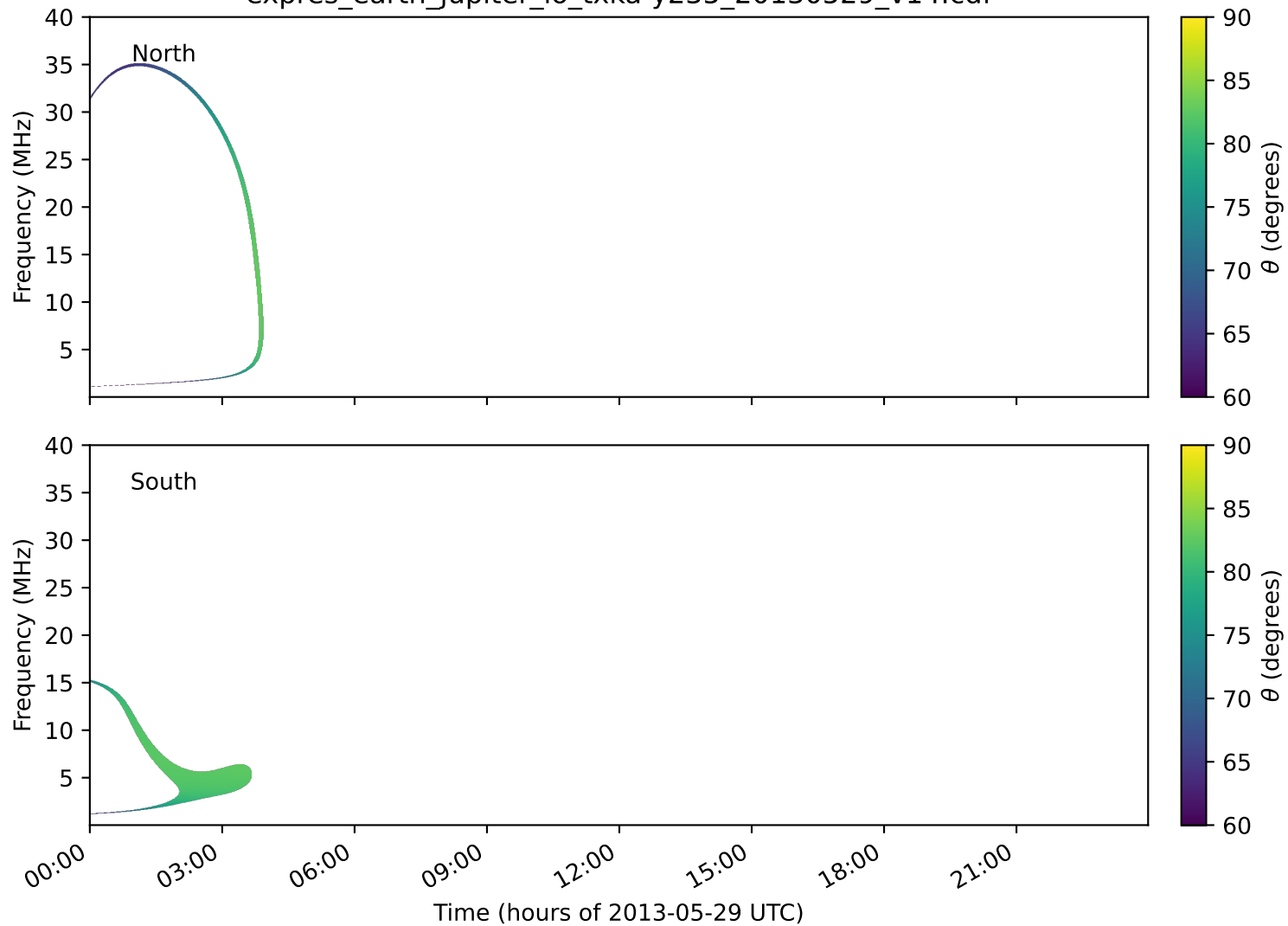
expres_earth_jupiter_io_txka-y235_20130529_v14.cdf
