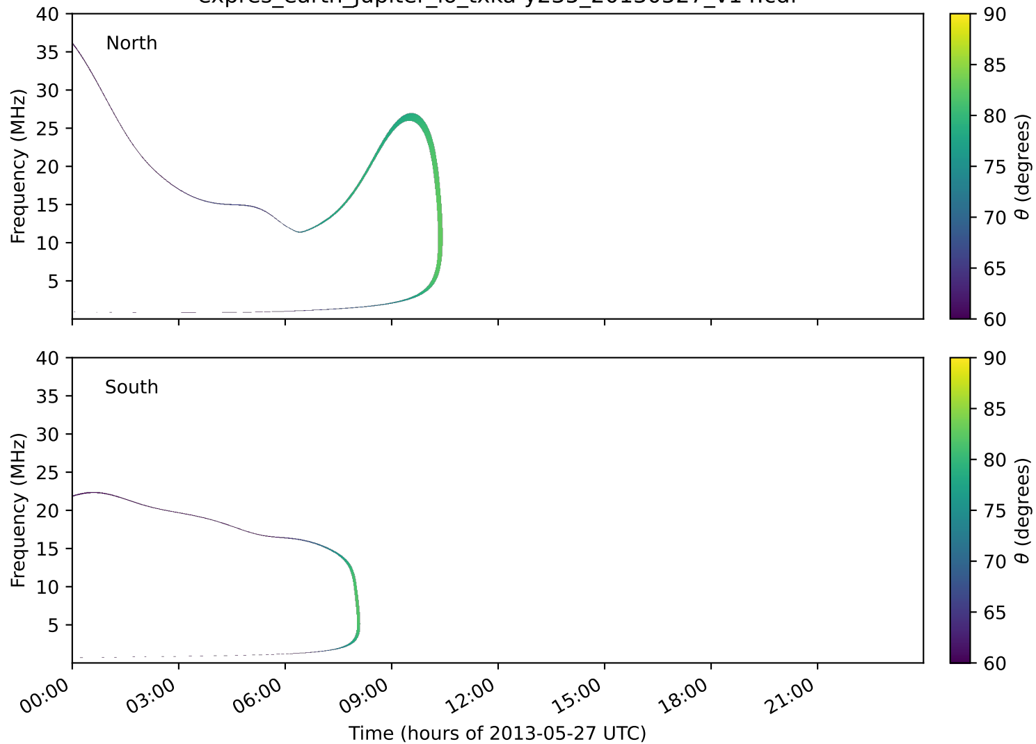
expres_earth_jupiter_io_txka-y235_20130527_v14.cdf
