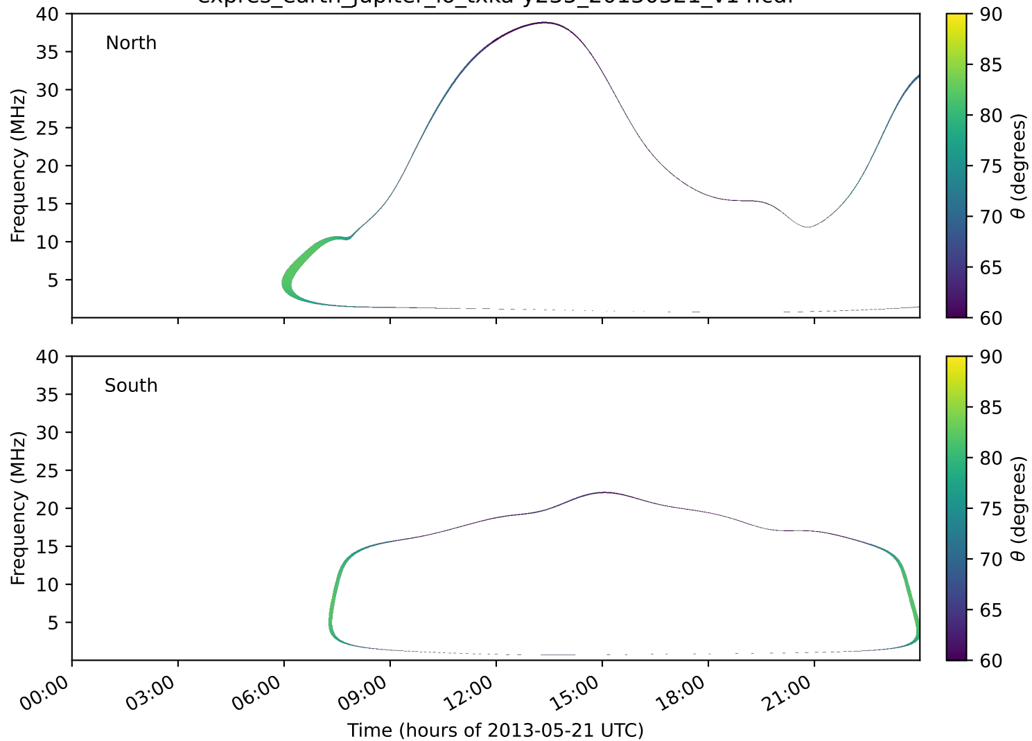
expres_earth_jupiter_io_txka-y235_20130521_v14.cdf
