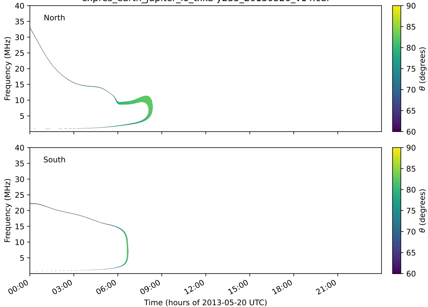
expres_earth_jupiter_io_txka-y235_20130520_v14.cdf
