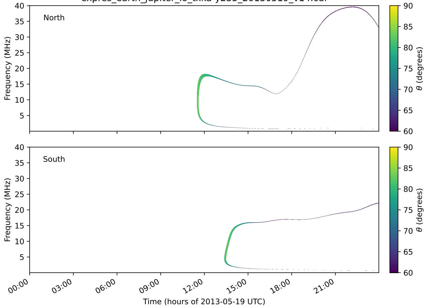
expres_earth_jupiter_io_txka-y235_20130519_v14.cdf
