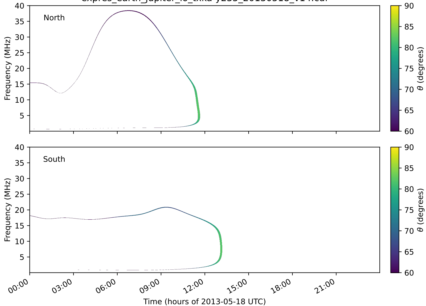
expres_earth_jupiter_io_txka-y235_20130518_v14.cdf
